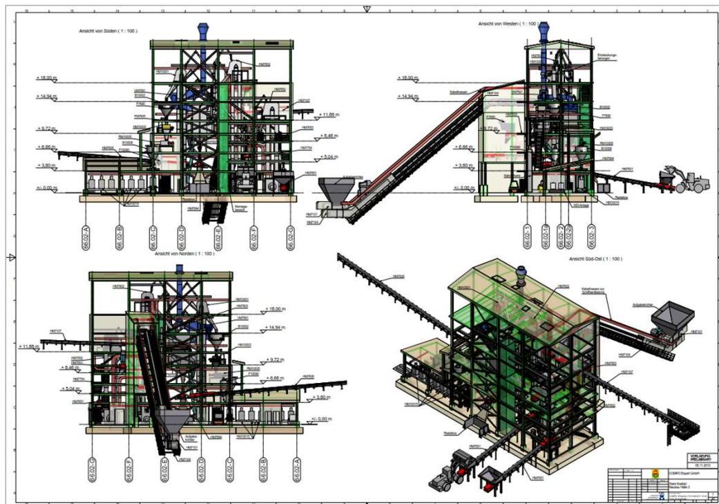
Layout plans
