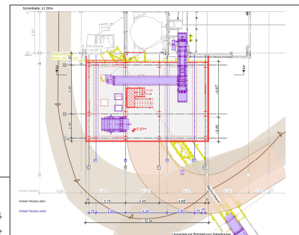
Layout designs
